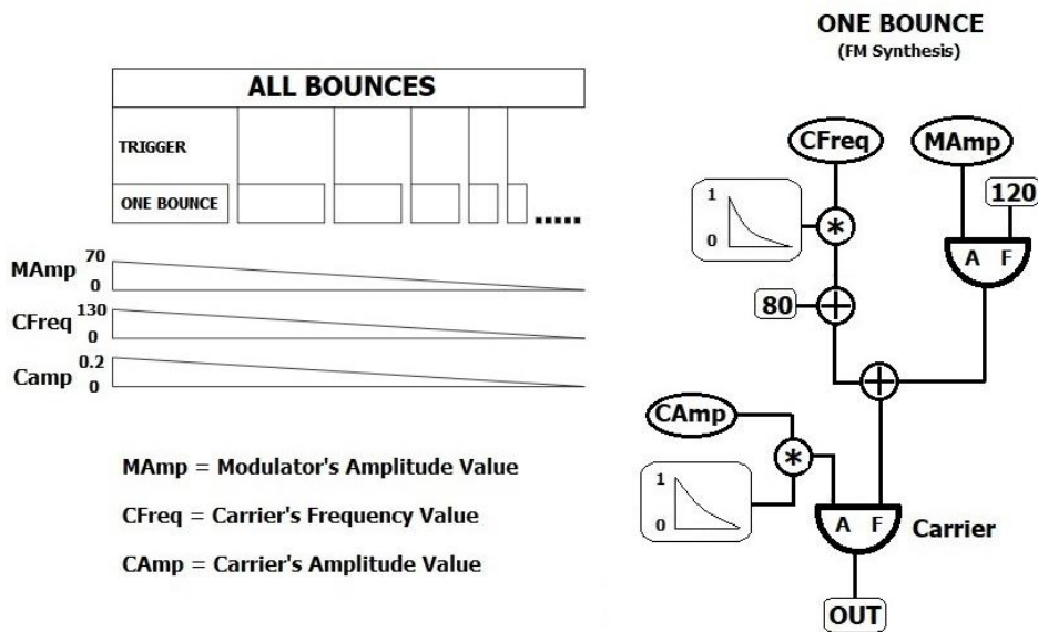
Fig. 2. Program diagrams
